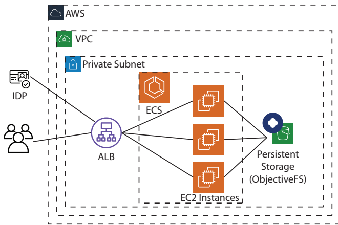
Fig. 1: Cloud Architecture.
