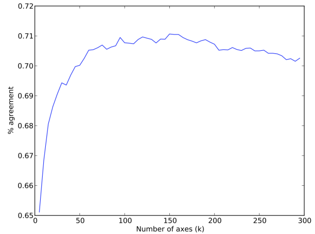
Fig. 2: Evaluating the predictive accuracy of the truncated SVD on ConceptNet for various values of k .
