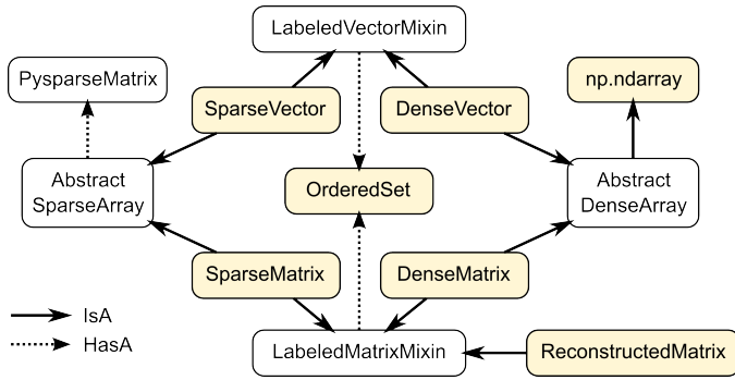
Fig. 1: Relationships between the main classes in Divisi 2.0, as well as some externally-defined classes.
